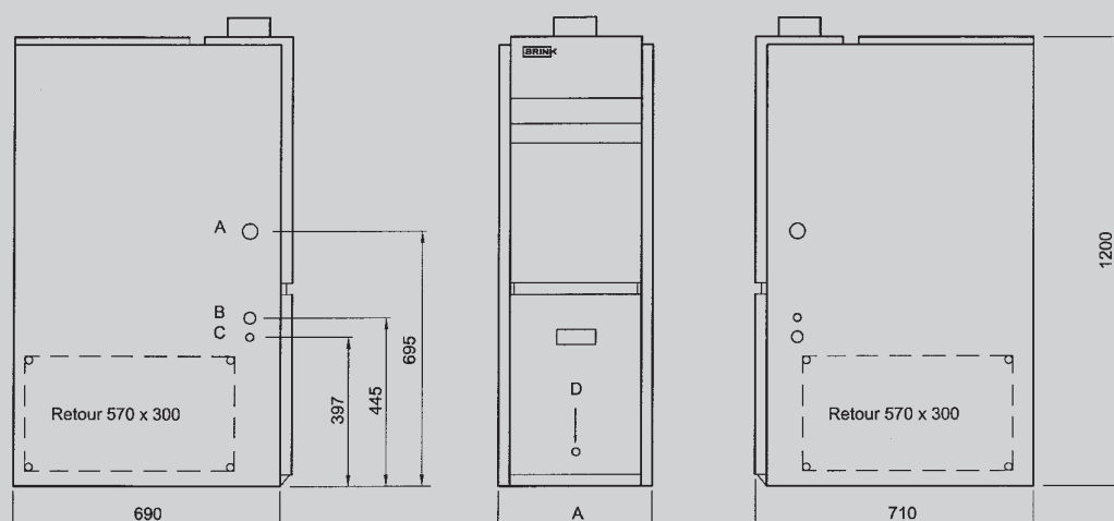
Figuur 3. Points de raccordement WG-N Upflow.
